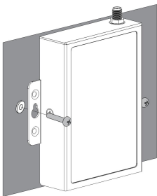
Wall Mounting
